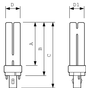
PL-C 18W/840/2P
