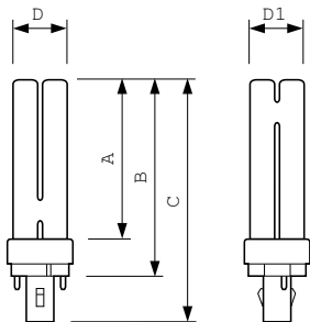
PL-C 18W/830/2P
